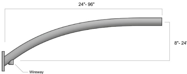
*48" arm with 12" rise shown
