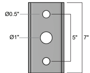
DRILLING DETAIL *Hardware by Others
